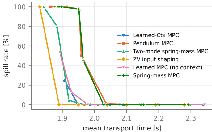
Nominal liquid (validation episodes)
