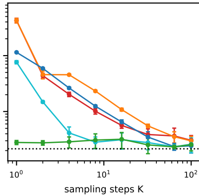
Moons
