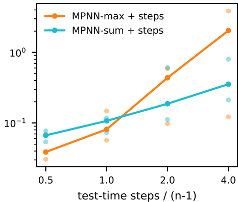
S16 MAE
