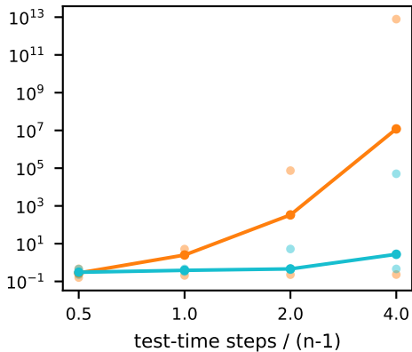
S64 MAE
