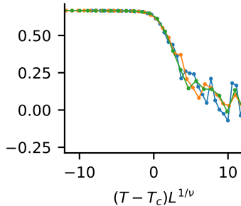
Binder U4 (seed 0)
