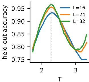
confusion W
