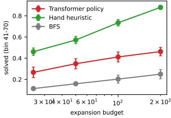
Fig. 3. Solved rate vs. expansion budget in the 41–70 bin (mean \pm std over seeds).
