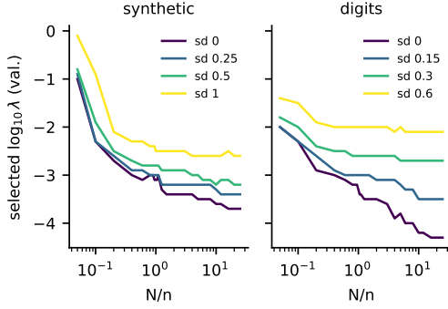
Fig. 3. Validation-selected \log_{10} \lambda against N/n for TunedRidge (mean of 5 seeds), by label-noise sd.
