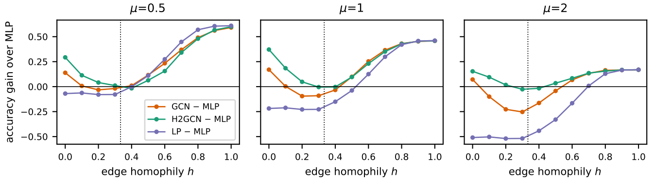
Fig. 3. Accuracy gain over the MLP for GCN, H2GCN-style and LP versus h (mean over 5 seeds). Values below zero mark where message passing hurts.
