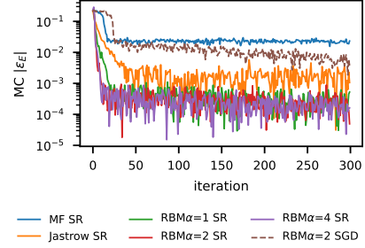
Fig. 2. MC energy error during training (10/1, start S).
