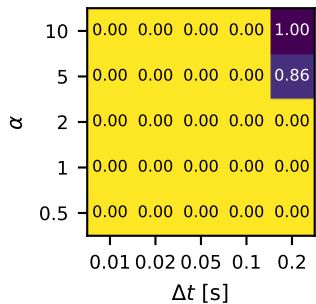
CT-CBF (Uni)
