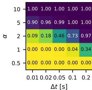
DT-CBF (Uni)
