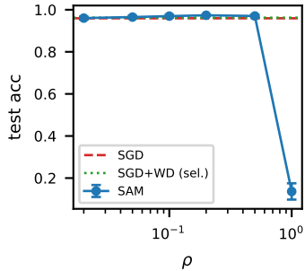
digits n0.0
