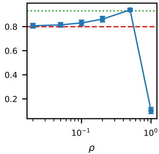
digits n0.2
