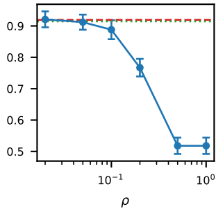
spirals n0.2
