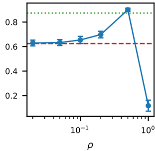
digits n0.4
