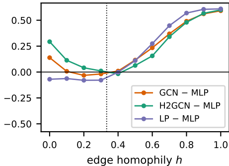
accuracy gain over MLP
