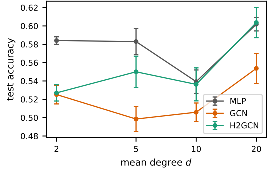
Fig. 2. Accuracy versus mean degree at h = 0.4 , \mu = 1 .
