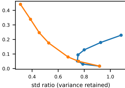
mode-weight TV
