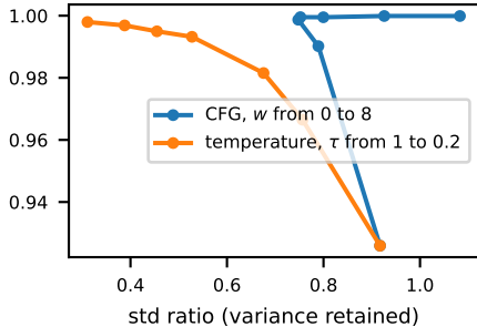
class accuracy
