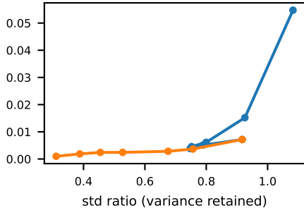
off-support mass
