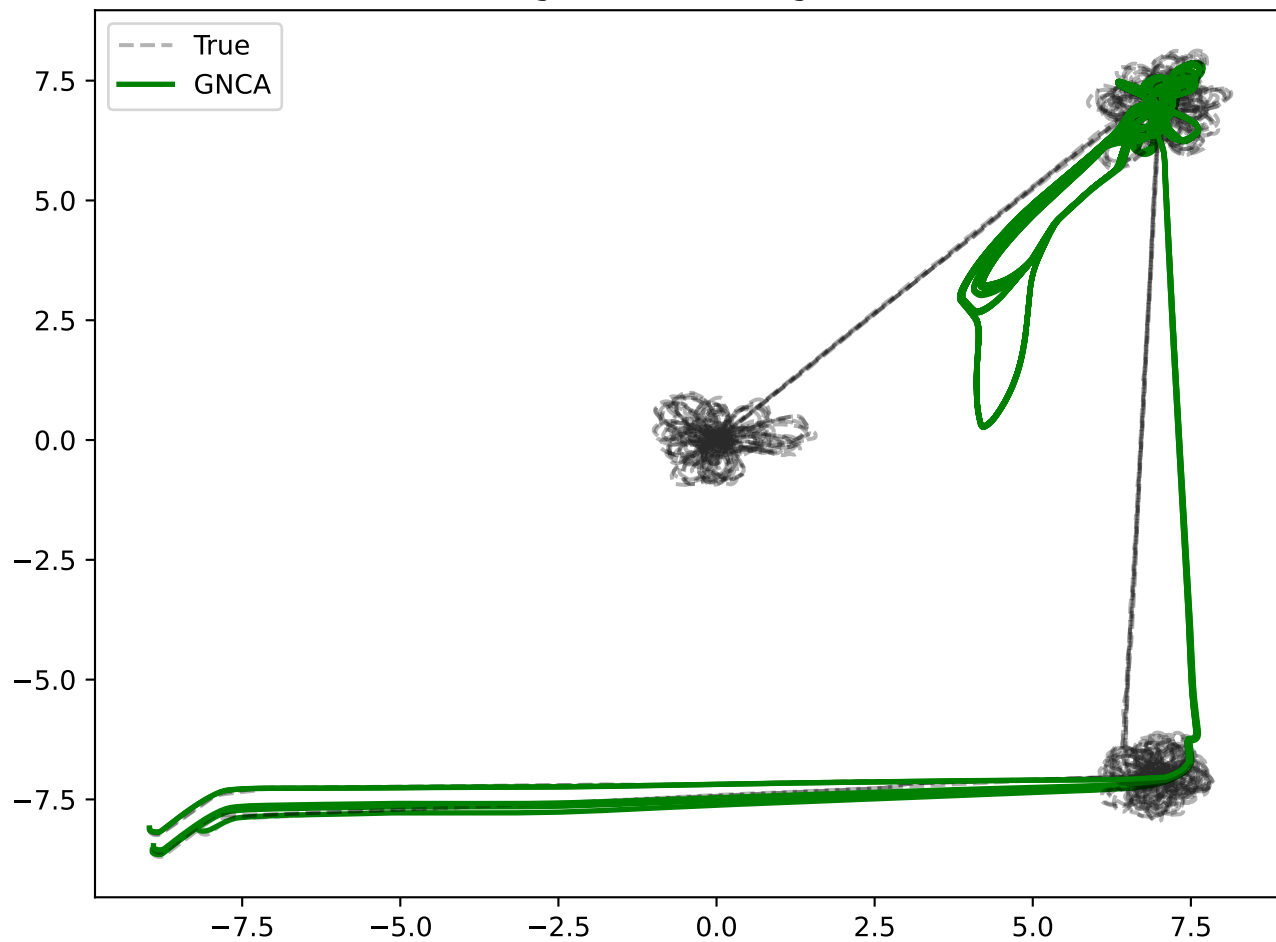
Autoregressive (Full Flight) Paths
