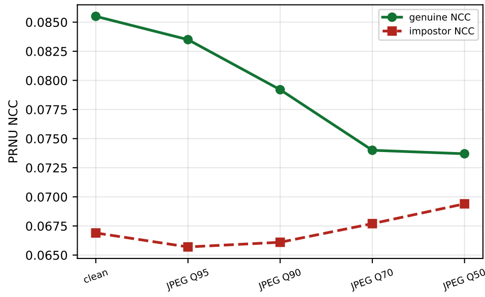
(d) Passive PRNU baseline: genuine-impostor margin shrinks under JPEG (motivates active mark)
