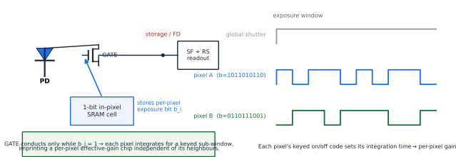
M2 — Coded-exposure pixel (per-pixel integration gating)
