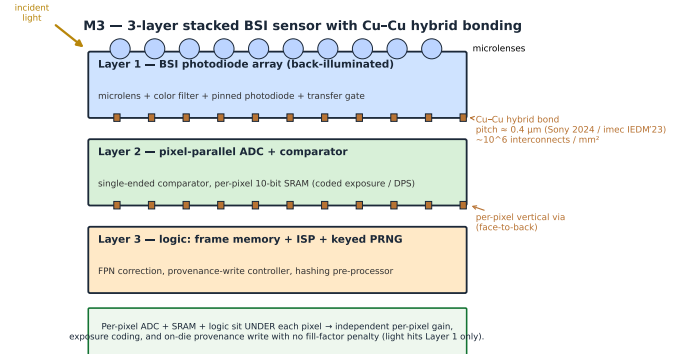
Fig. 5. M3: a 3-layer stacked BSI sensor joined by Cu–Cu hybrid bonding ( \approx 0.4\mu\text{m} pitch, \sim 10^6 interconnects/ \text{mm}^2 ). A per-pixel ADC, SRAM, and a logic tier (frame memory, ISP, keyed PRNG/provenance-write) sit under each pixel with no fill-factor penalty.
