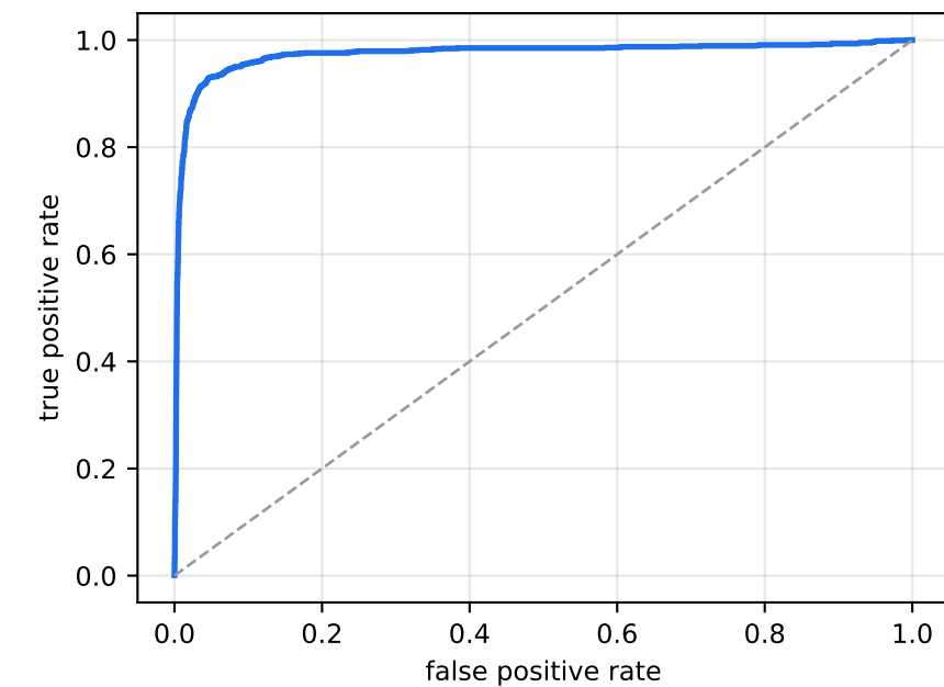
(c) Tamper-localization ROC (real splices) block-level, AUC \approx 0.97
