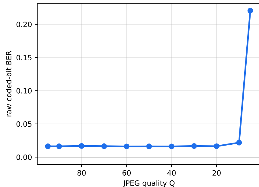
(a) In-pixel channel BER vs real-JPEG quality (Kodak, pre-ECC; RS recovers payload \geq Q10)
