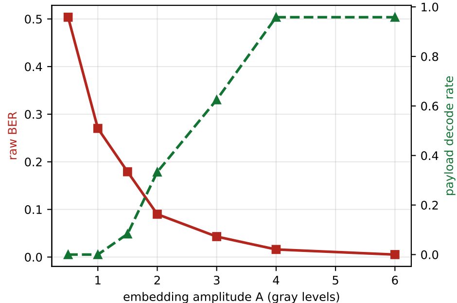
(b) Amplitude operating curve @ JPEG Q40 (genuine robustness cliff on real images)
