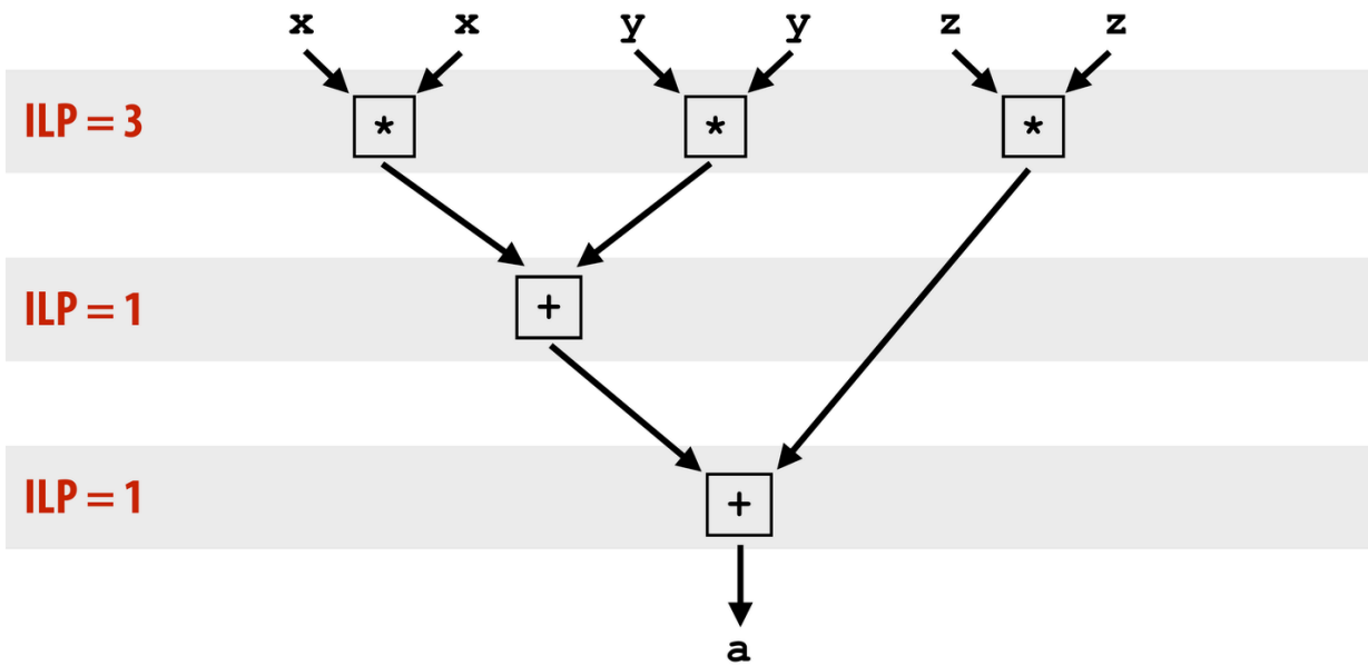
DEPENDENCY GRAPH FOR a = x^2 + y^2 + z^2 . CRITICAL-PATH LENGTH THREE — THE MINIMUM CYCLE COUNT REGARDLESS OF ISSUE WIDTH.
