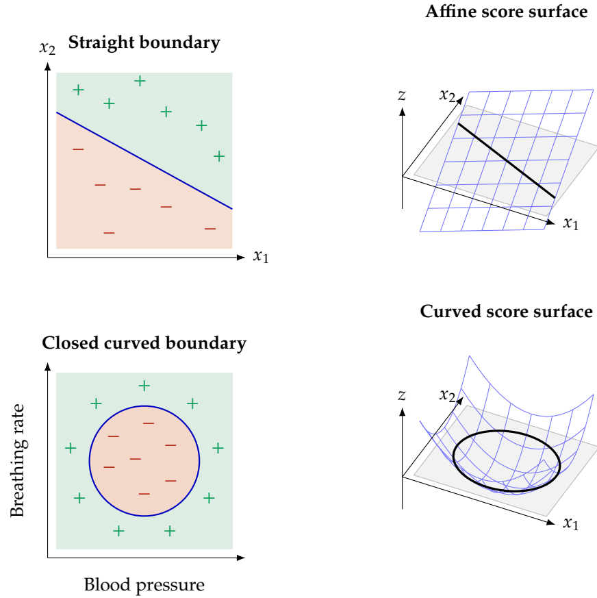
Figure 14: Schematic boundaries and score surfaces. An affine score gives a straight zero boundary; a bowl-shaped score gives a closed curved boundary. Intersecting a score surface with z = 0 identifies the classification boundary.
