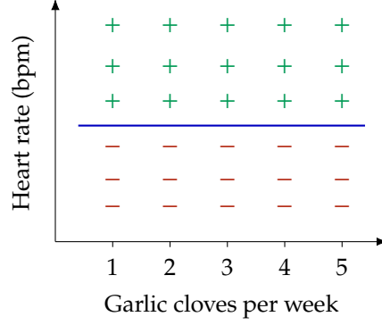
Figure 11: Schematic heart rate and garlic-consumption example. The horizontal boundary ignores the horizontal feature. No measured heart rates are implied.
