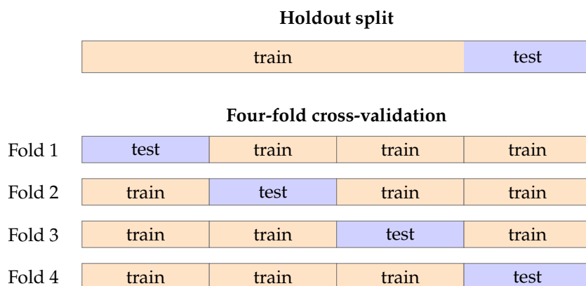
Figure 16: A schematic holdout split and four-fold cross-validation. Blue marks held-out data; pale orange marks training data. In each fold the blue chunk changes, and a fresh classifier is trained on the other chunks.
