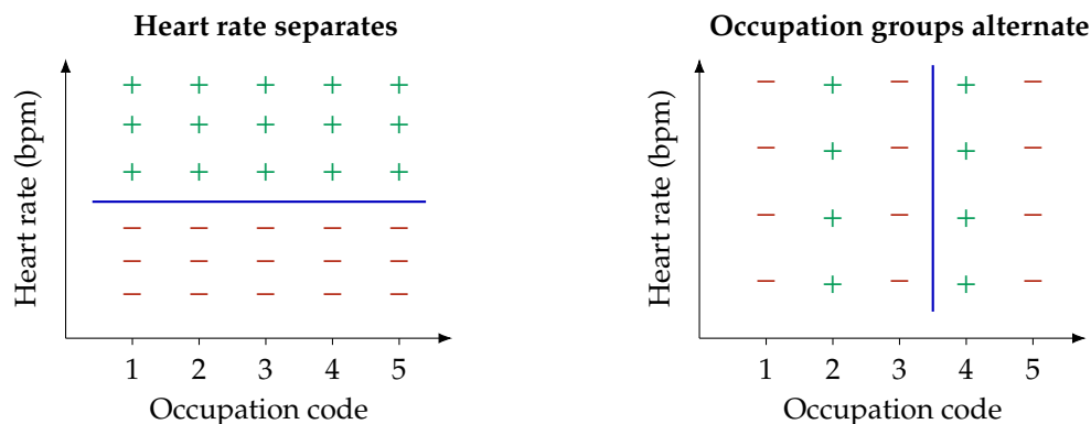
Figure 9: Schematic occupation and heart-rate arrangements. A horizontal line separates the left arrangement. On the right, doctors and pharmacists are positive while the other occupations are negative. One straight boundary cannot alternate between these groups at the same heart rate. The displayed candidate line illustrates the mismatch.
