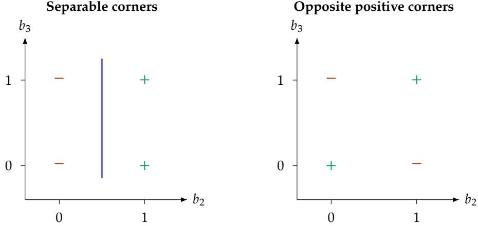
Figure 10: Schematic labels on the four binary-code corners. The left pattern is separated by b_2 = 1/2 . The right pattern has positive opposite corners; no straight line strictly separates it. Distinct codes alone do not ensure that a linear classifier can express the desired categories.
