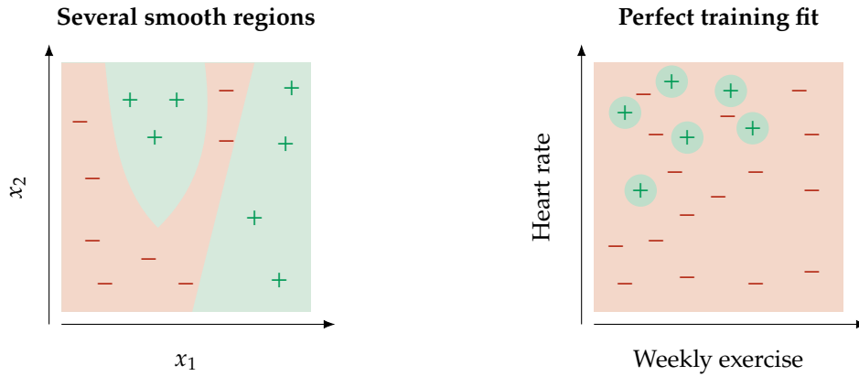
Figure 15: Schematic effects of flexible boundaries. The left panel shows several regions defined by a smooth score. On the right, small positive islands fit every training label in the heart-rate and exercise example. Zero training error leaves performance on new examples unresolved.
