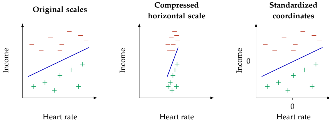
Figure 12: Schematic income and heart-rate geometry: changing the horizontal scale compresses the points and rotates the displayed boundary. Standardized coordinates put the features on comparable scales, with zero at each mean. The panels illustrate representations, not additional measurements.
