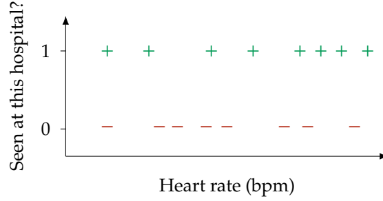
Figure 13: Schematic hospital indicator versus heart rate. The indicator alone separates these labels, making its meaning an essential part of interpretation.
