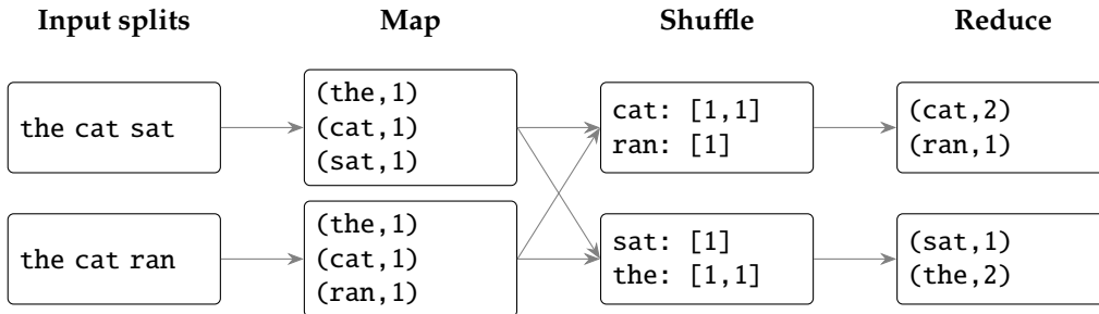
Figure 1: Word count with M = 2 map tasks and R = 2 reduce tasks. Each mapper emits (w, 1) per word; the shuffle sends every pair with key w to partition \text{hash}(w) \bmod R and groups its values; each reducer sums the list for each of its keys.
