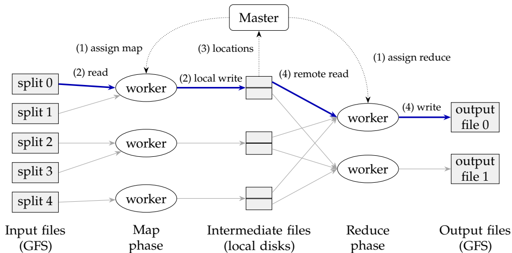
Figure 2: MapReduce execution. The master assigns tasks (1); each map worker reads a split and writes R partitioned regions to its local disk (2) and reports their locations (3); each reduce worker fetches its region from every map worker and writes one output file (4). The highlighted path follows the records of split 0 destined for partition 0.
