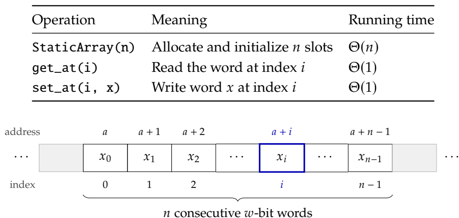
Figure 1: A static array of length n occupies n consecutive w -bit words starting at address a . Slot i lives at address a + i , so get_at(i) and set_at(i, x) each touch one word in \Theta(1) time.
