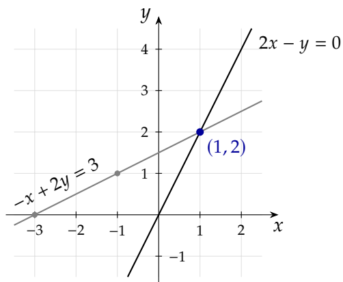
Figure 1: Row picture: the lines 2x - y = 0 and -x + 2y = 3 meet at (1, 2) .
