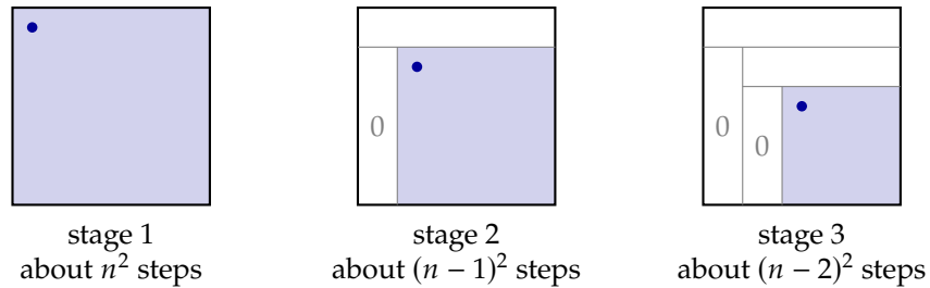
Figure 5: Elimination on a dense n -by- n matrix. Each stage works only on the shaded block, whose top row holds the current pivot (dot); the block shrinks by one row and one column from stage to stage, leaving zeros below the earlier pivots.
