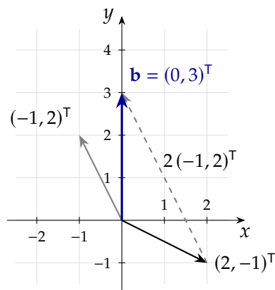
Figure 2: Column picture: one copy of (2, -1)^T plus two copies of (-1, 2)^T gives \mathbf{b} = (0, 3)^T .
