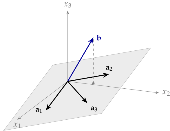
Figure 3: Three dependent columns \mathbf{a}_1 , \mathbf{a}_2 , \mathbf{a}_3 of a singular 3-by-3 matrix lie in one plane through the origin. Every combination stays in that plane, so a right-hand side \mathbf{b} off the plane cannot be reached.
