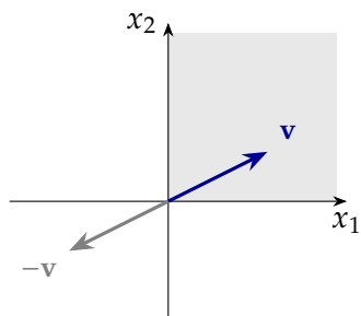
Figure 6: The positive quadrant (shaded) contains \mathbf{v} but not -\mathbf{v} , so it is not closed under scalar multiplication.
