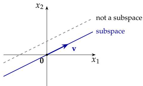
Figure 7: The multiples c\mathbf{v} fill a line through the origin, a subspace of \mathbb{R}^2 . The parallel dashed line misses \mathbf{0} .
