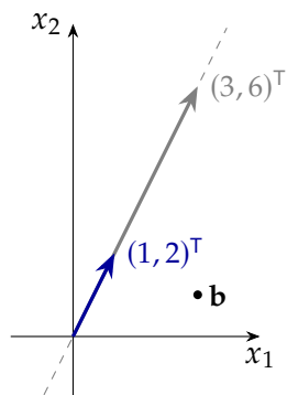
Figure 4: The columns (1, 2)^T and (3, 6)^T of the singular matrix lie on one line through the origin. Every combination stays on that line, so a right-hand side such as \mathbf{b} off the line cannot be reached.
