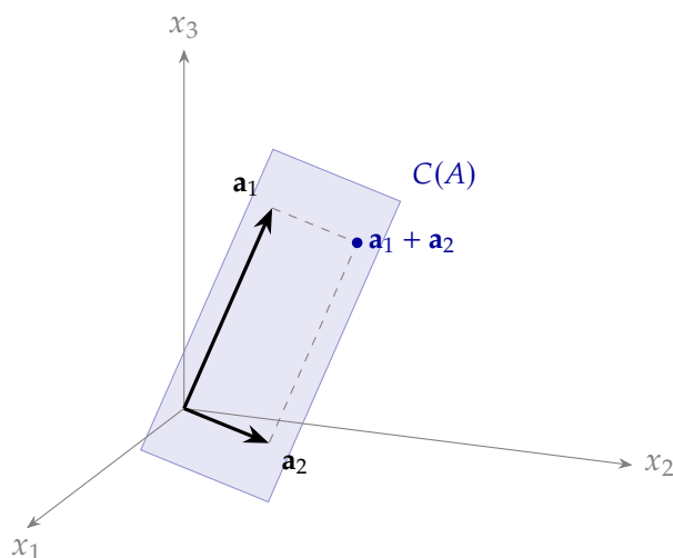
Figure 8: The column space C(A) of the 3-by-2 example is the plane through the origin spanned by \mathbf{a}_1 = (1, 2, 4)^T and \mathbf{a}_2 = (3, 3, 1)^T . Every combination, such as \mathbf{a}_1 + \mathbf{a}_2 = (4, 5, 5)^T , lies in it, and A\mathbf{x} = \mathbf{b} is solvable only for \mathbf{b} in this plane.
