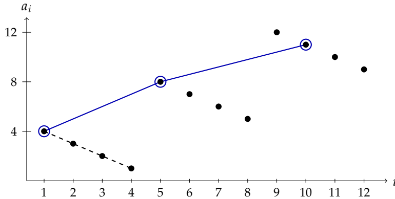
Figure 1: The sequence 4, 3, 2, 1, 8, 7, 6, 5, 12, 11, 10, 9 plotted as points (i, a_i) . The solid path marks the increasing subsequence 4, 8, 11 and the dashed path the decreasing subsequence 4, 3, 2, 1; neither can be lengthened.
