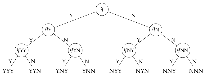
Figure 2: A deterministic adaptive strategy with three questions. The question asked next depends only on the answers so far, so each object that reaches a leaf is identified by its answer history. With twenty questions the tree has 2^{20} leaves.
