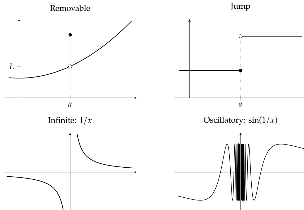
Figure 3: The four kinds of discontinuity at a point a (at a = 0 in the bottom row). An open circle marks a point excluded from the graph, and a filled circle marks the assigned value.
