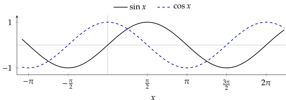
Figure 6: The graphs of \sin x and \cos x . The slope of \sin x at each point is the height of \cos x , and the slope of \cos x is the height of -\sin x .
