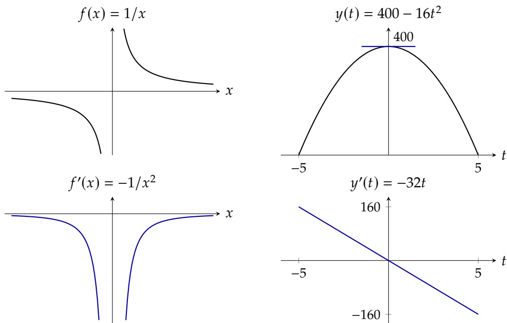
Figure 4: Functions (top) and their derivatives (bottom). Left: the odd function 1/x has the even, everywhere negative derivative -1/x^2 . Right: the height 400 - 16t^2 has velocity -32t , which is zero where the tangent line is horizontal at the top of the path.
