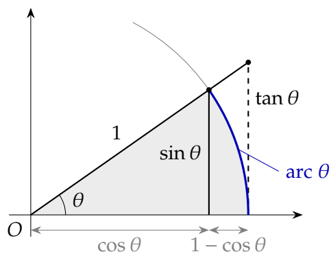
Figure 5: An angle \theta at the center of the unit circle. The vertical side \sin \theta , the arc of length \theta (highlighted), and the tangent segment \tan \theta satisfy \sin \theta < \theta < \tan \theta ; the horizontal gap 1 - \cos \theta is much smaller than \theta when \theta is small.
