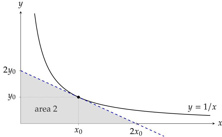
Figure 2: The tangent line to y = 1/x at (x_0, y_0) , where y_0 = 1/x_0 , meets the axes at 2x_0 and 2y_0 . The shaded triangle always has area 2.
