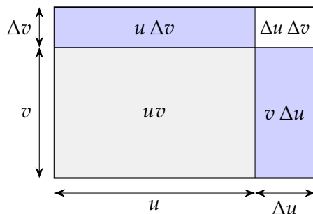
Figure 7: Growing the sides of a u -by- v rectangle by \Delta u and \Delta v adds two strips of areas u \Delta v and v \Delta u (shaded) and a corner of area \Delta u \Delta v , which is negligible for small changes.
