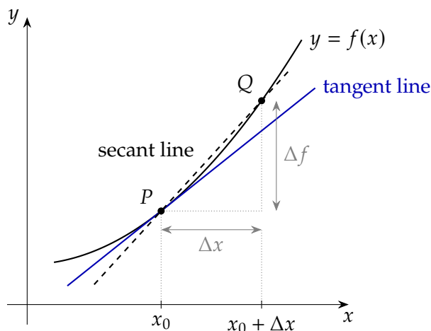
Figure 1: The secant line through P = (x_0, f(x_0)) and Q = (x_0 + \Delta x, f(x_0 + \Delta x)) has slope \Delta f / \Delta x . As \Delta x \rightarrow 0 , Q moves toward P and the secant lines approach the tangent line at P .
