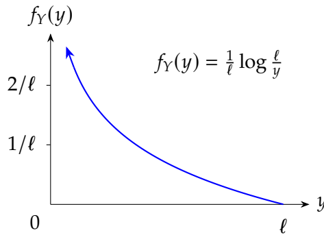
Figure 41: The second break's density decreases toward zero at \ell and grows without bound near zero. The plotted portion follows \ell f_Y(y) = \log(\ell/y) ; the upward arrow indicates the omitted continuation near zero.
