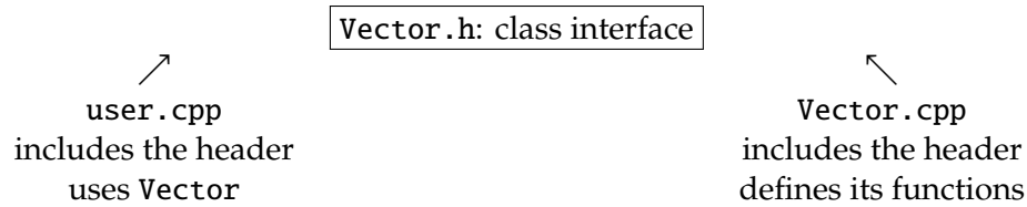
Figure 4: Client and implementation share a header and compile as separate translation units.
