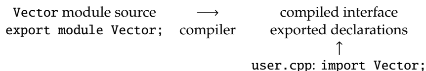
Figure 5: A module's compiled interface supplies the declarations used by importing clients.
