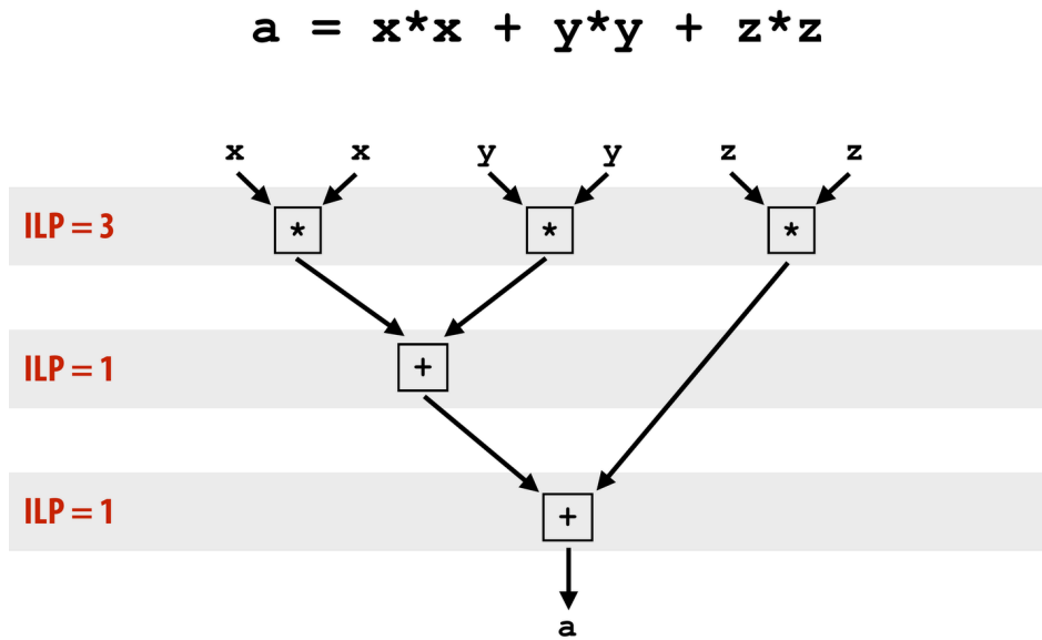
Dependency graph for a = x^2 + y^2 + z^2 . Critical-path length three — the minimum cycle count regardless of issue width.
