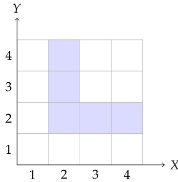
Figure 1: The sample space for two rolls of a tetrahedral die, with X the first roll and Y the second. The five shaded cells are the event \{\min(X, Y) = 2\} .
