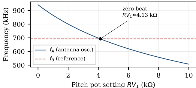
(b) Coarse tuning by the pitch pot
