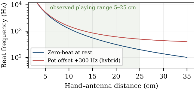
(a) Pitch vs. distance (model)
