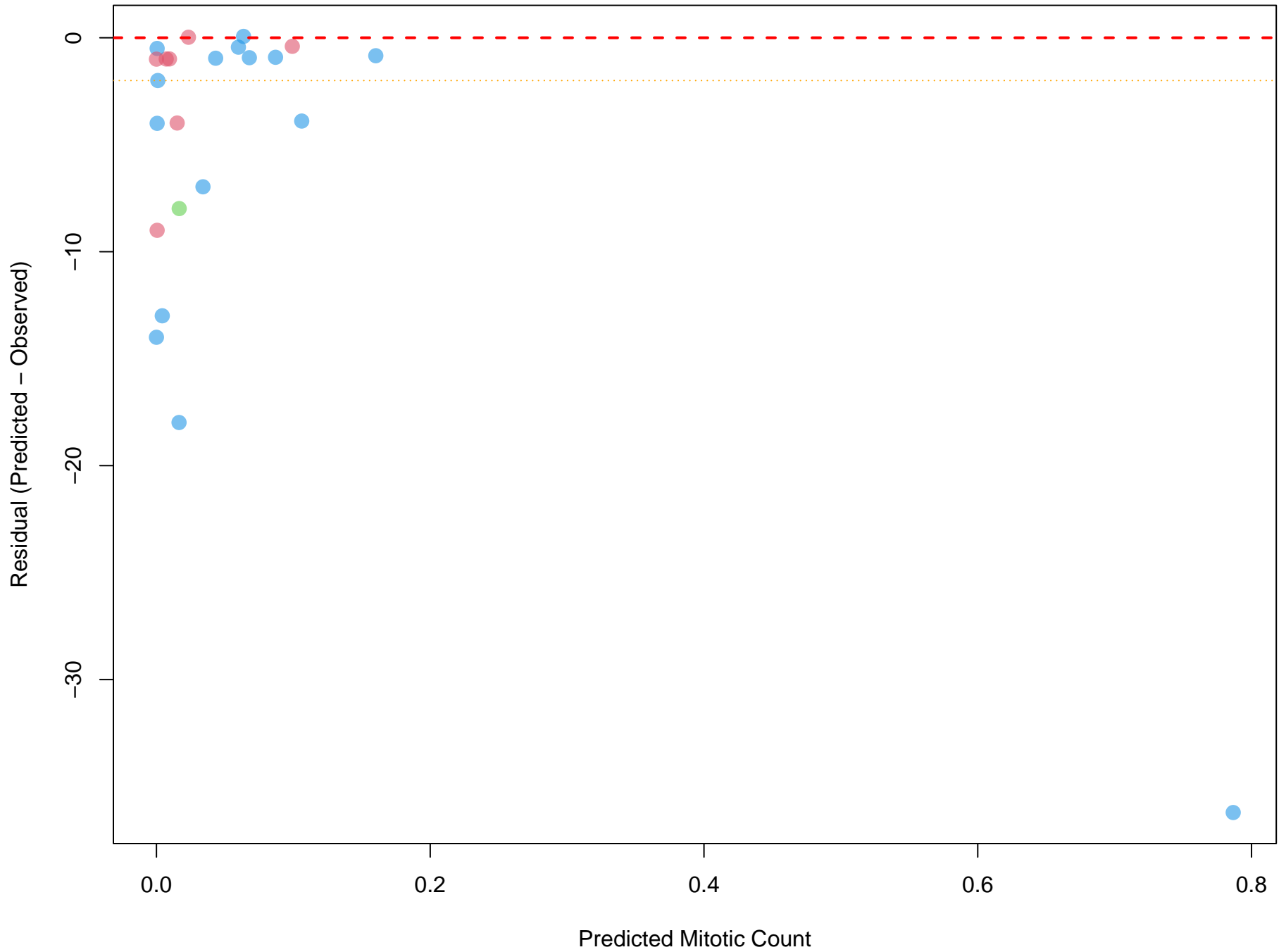
Residual Plot
