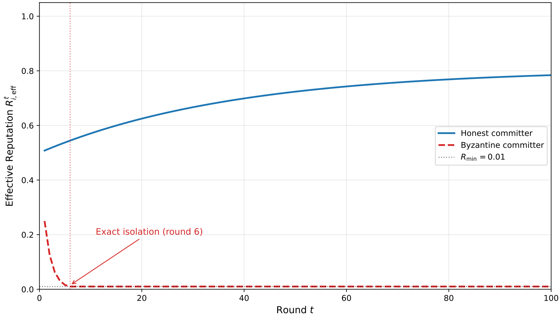
Figure 2: Reputation Convergence (Canonical State Machine)
