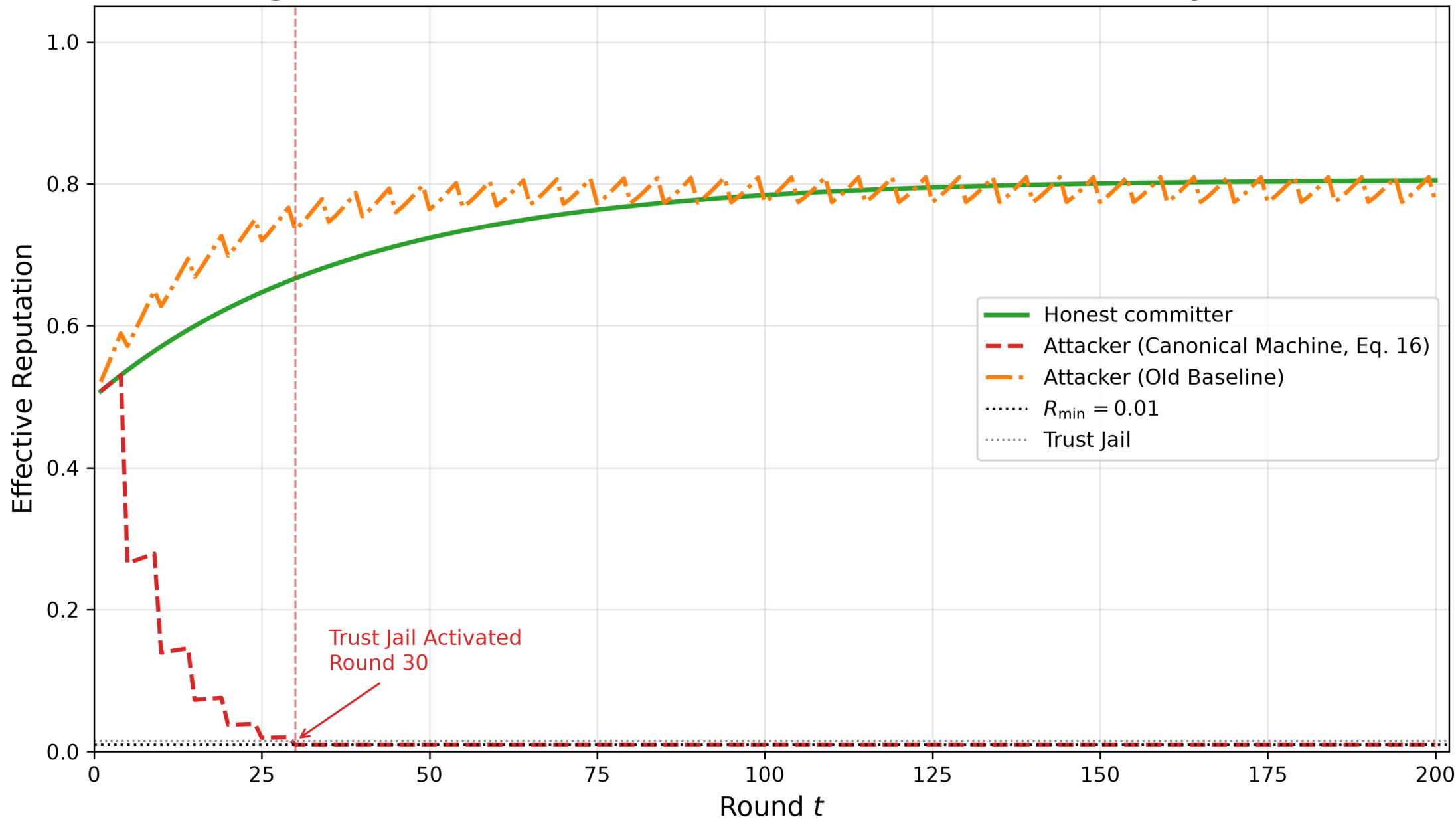
Figure 3b: Slow-Loris Attack Defeated via Geometric Safety Slash
