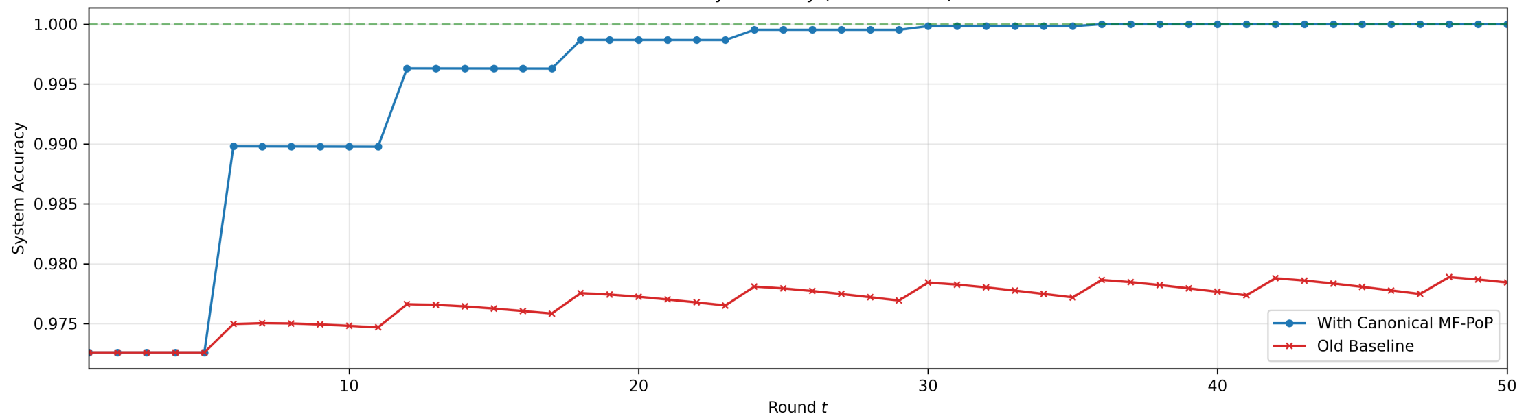
Accuracy Recovery (Rounds 1-50)
