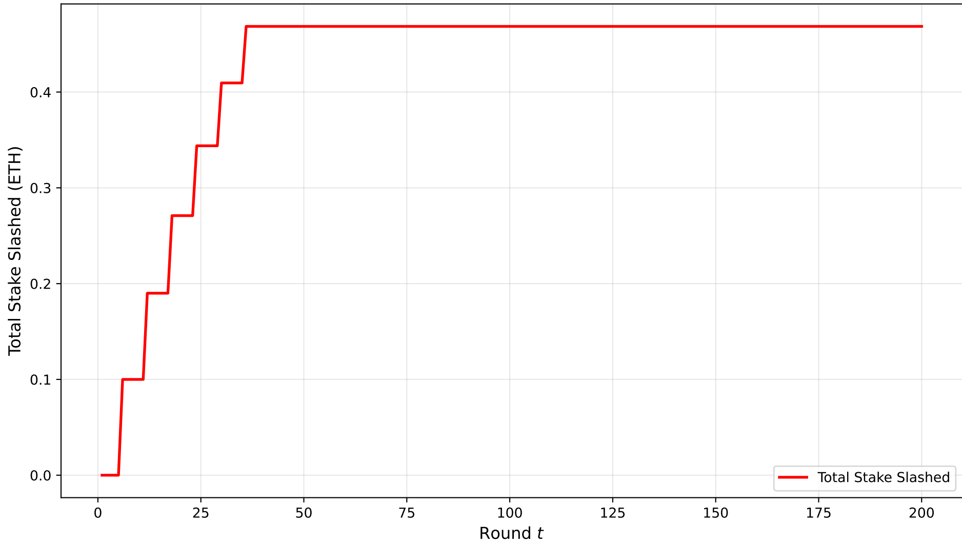
Cumulative Stake Slashing Under Canonical MF-PoP
