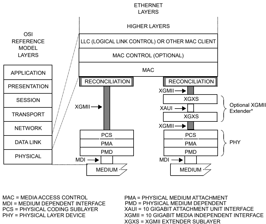
Figure 46–1—XGMII relationship to the ISO/IEC Open Systems Interconnection (OSI) reference model and the IEEE 802.3 Ethernet model
