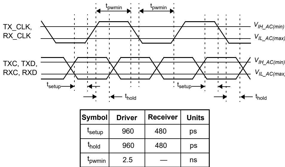
Figure 46-16—TX_CLK and RX_CLK timing parameters
