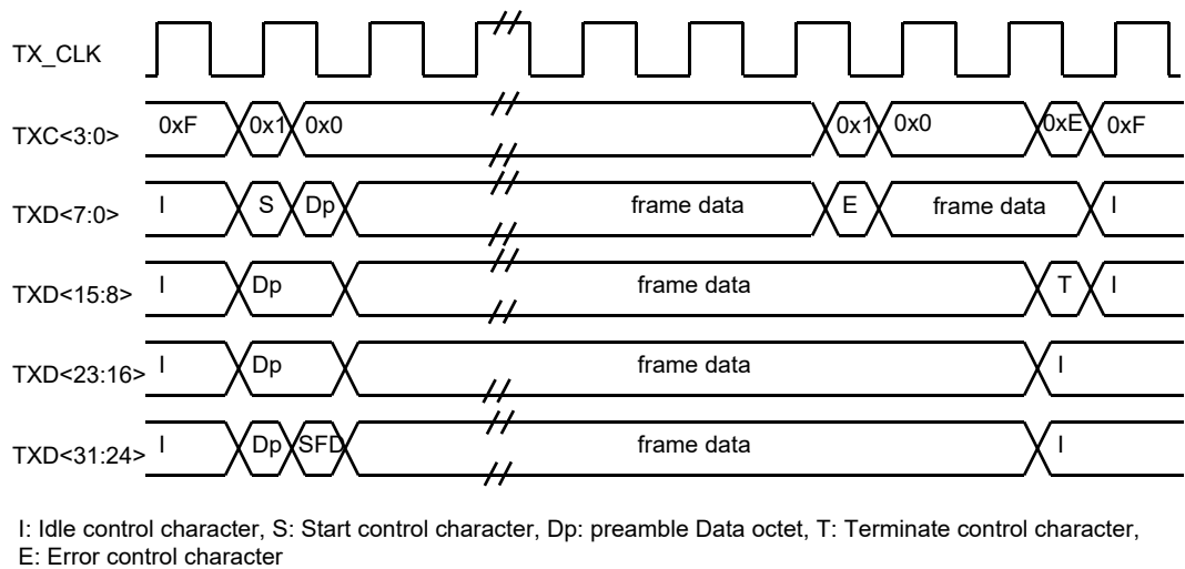
Figure 46–6—Transmit Error Propagation
