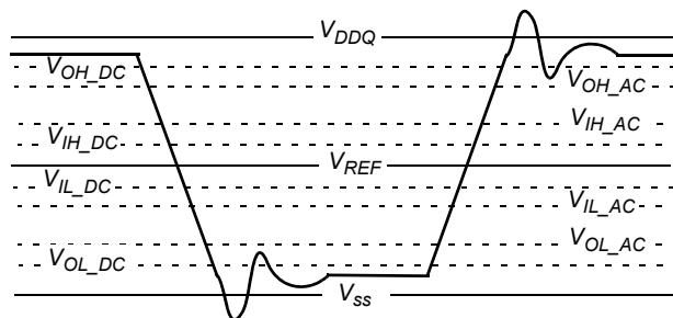
Figure 46–14—Electrical characteristics (illustrative)
