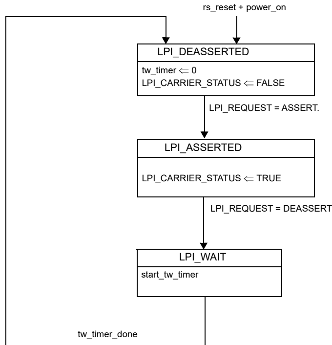
Figure 46–13—Transmit LPI state diagram
