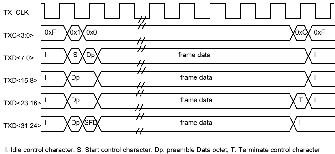
Figure 46–5—Normal frame transmission
