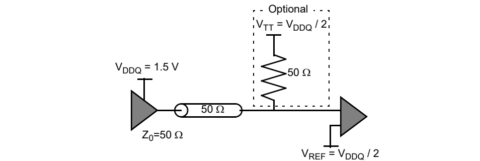
Figure 46-15—Circuit topology example
