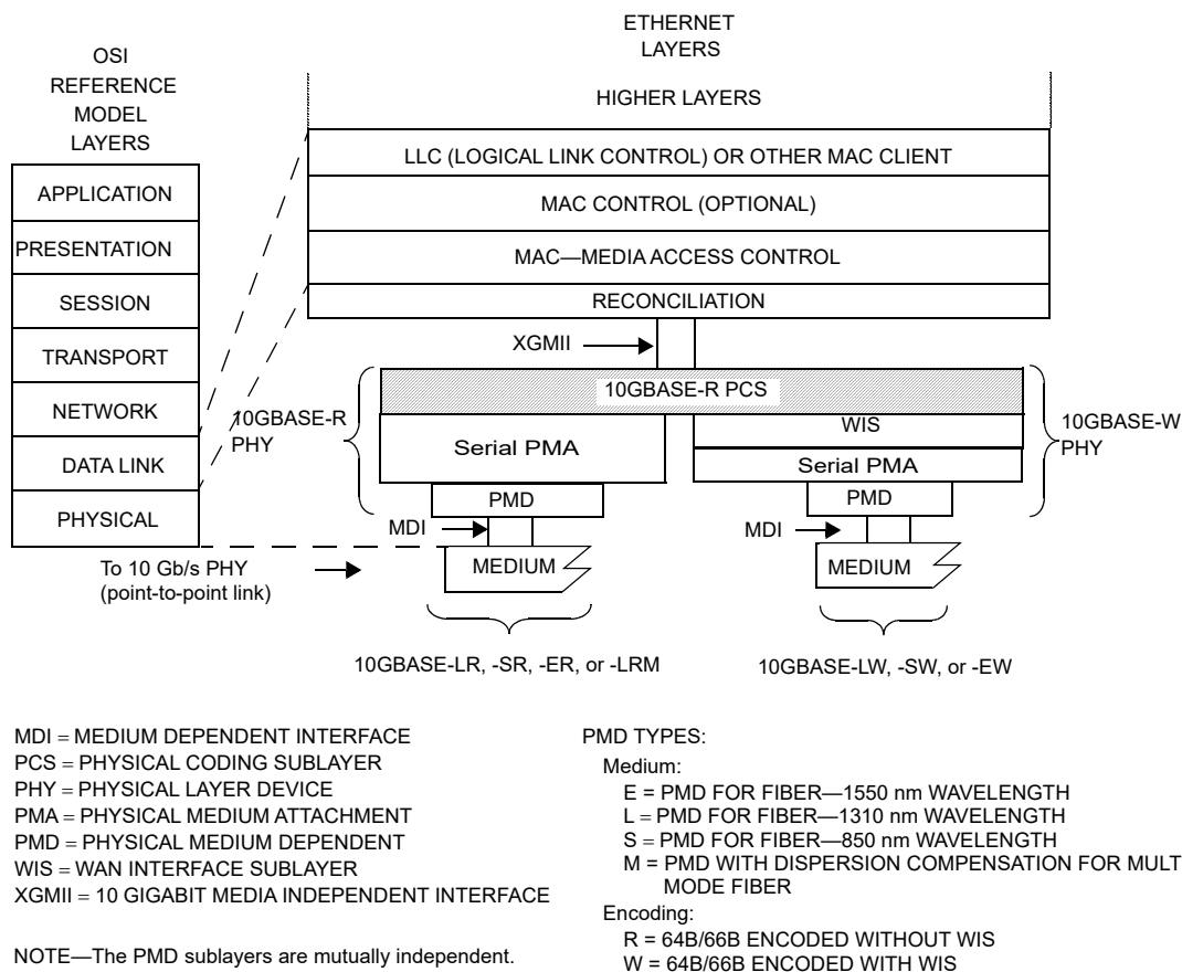
Figure 49–1—10GBASE-R PCS relationship to the ISO/IEC Open Systems Interconnection (OSI) reference model and IEEE 802.3 Ethernet model
