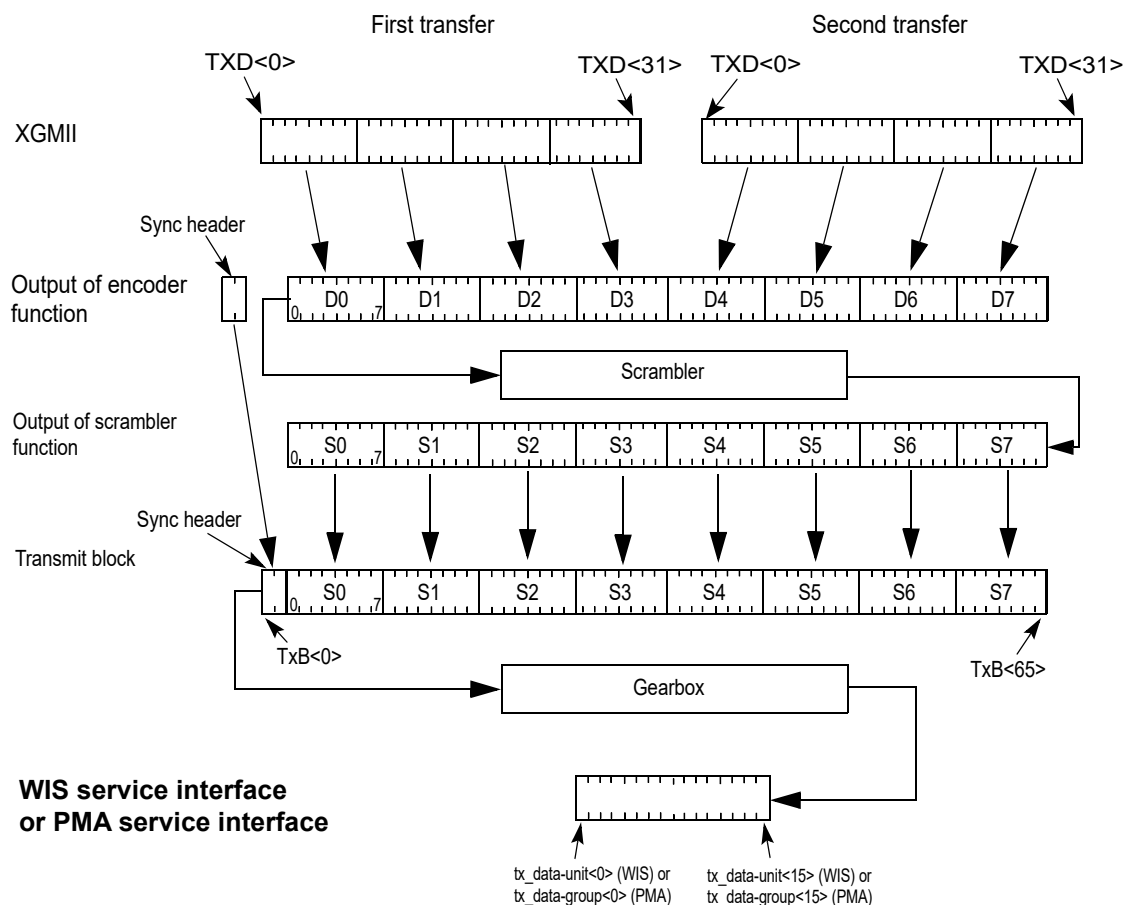
Figure 49-5—PCS Transmit bit ordering
