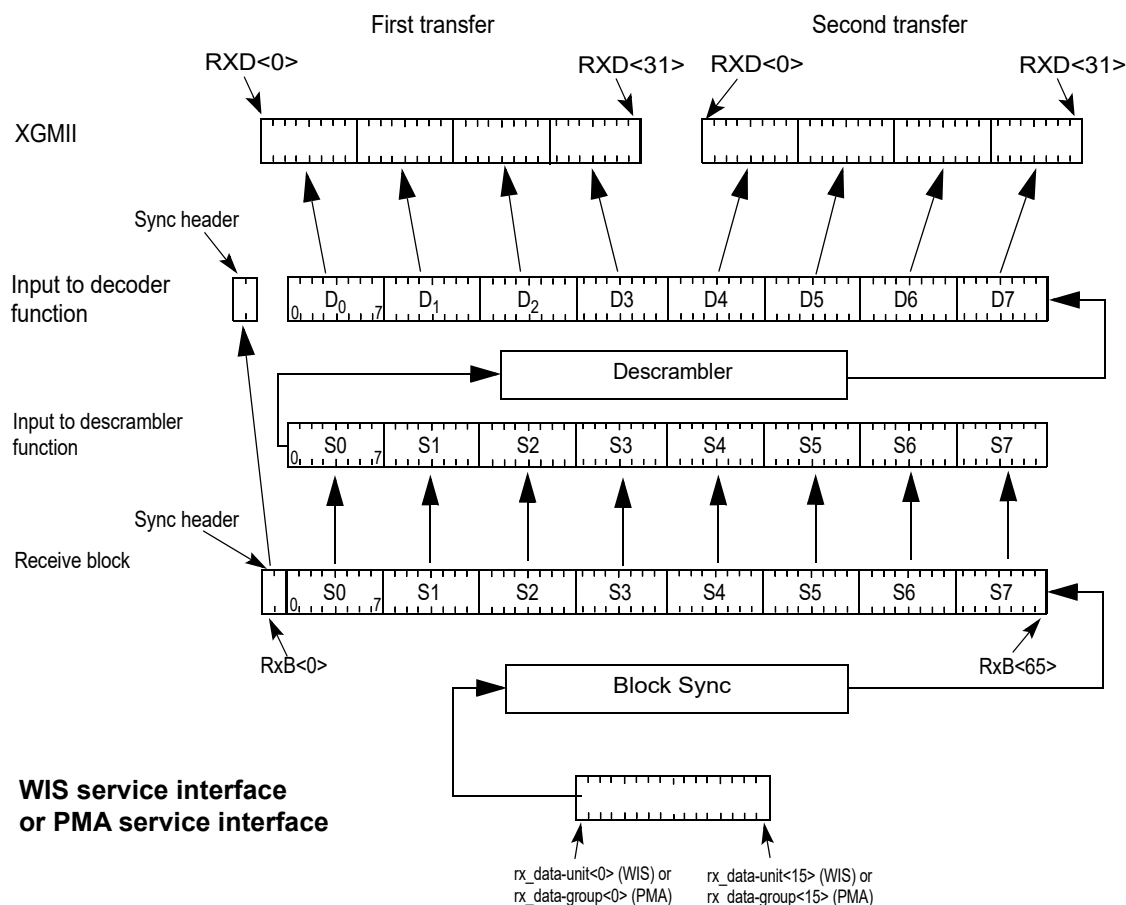
Figure 49-6—PCS Receive bit ordering
