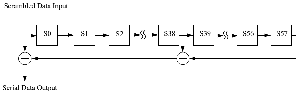
Figure 49-10—Descrambler
