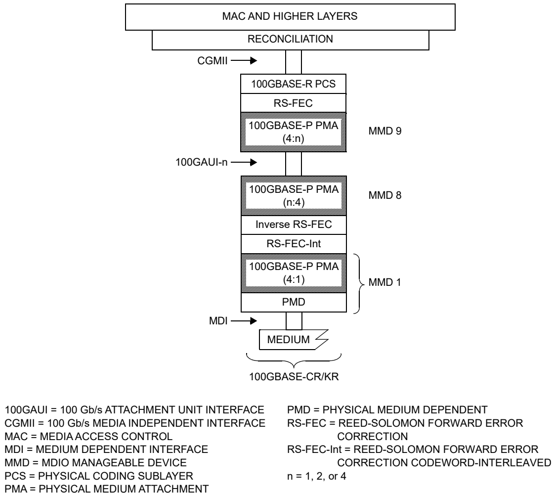
Figure 135A–7a—Example 100GBASE-CR/KR PHY with RS-FEC and RS-FEC-Int
