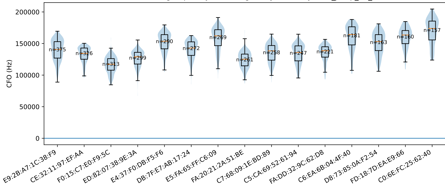
Transition CFO grouped by AdvA (tag ecosystem only): cfo_jump_10_hz
