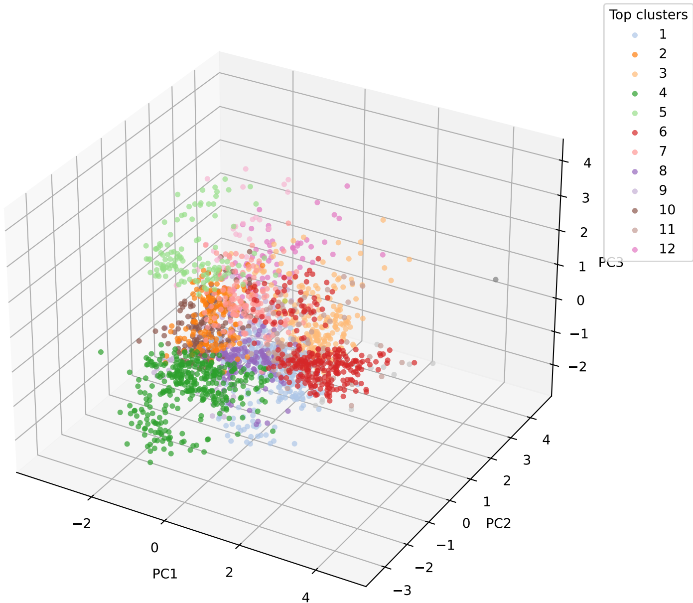
Clusters in 3-D PCA space (EVR: 0.33, 0.32, 0.24)
