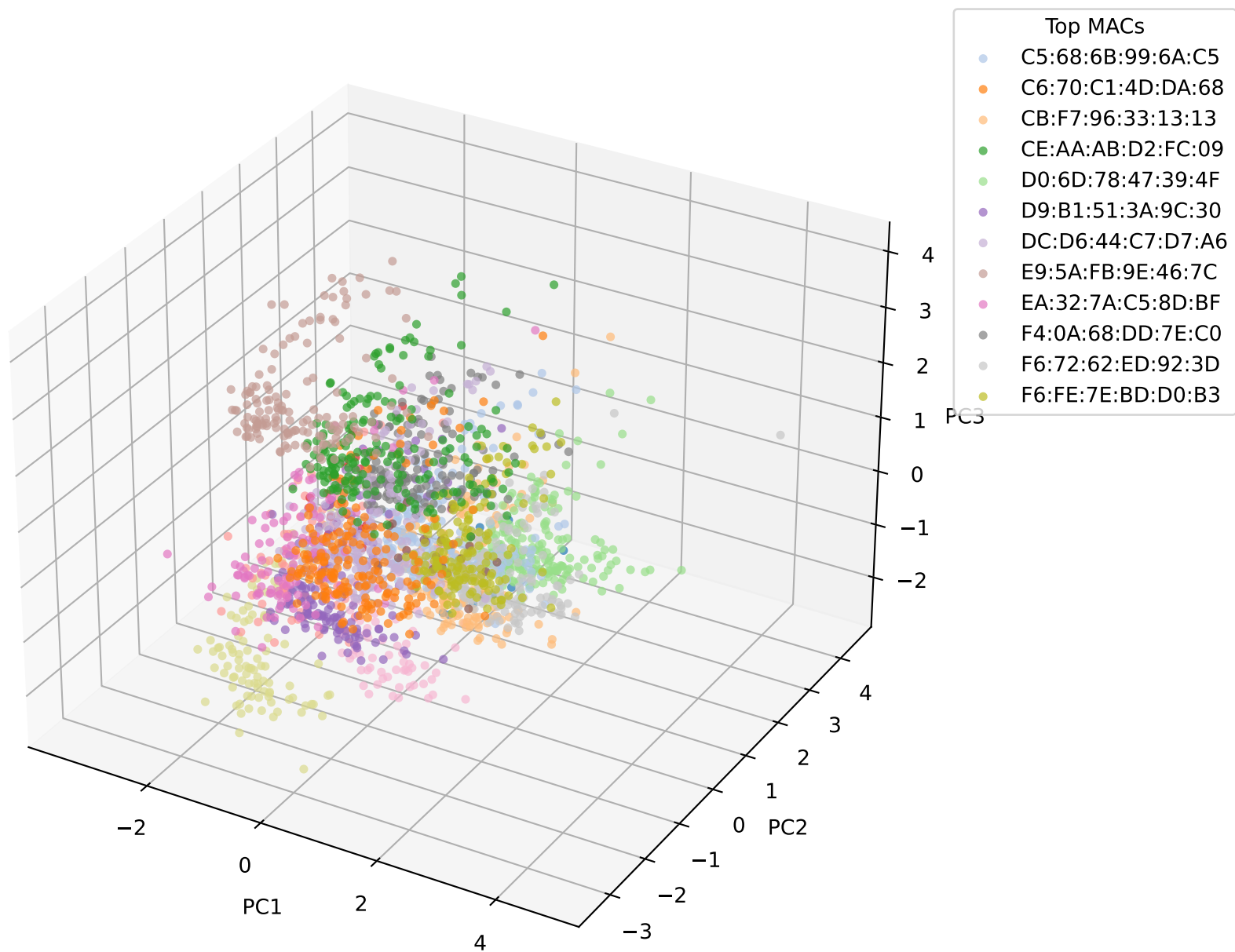
MAC-colored 3-D PCA of CFO (EVR: 0.33, 0.32, 0.24)
