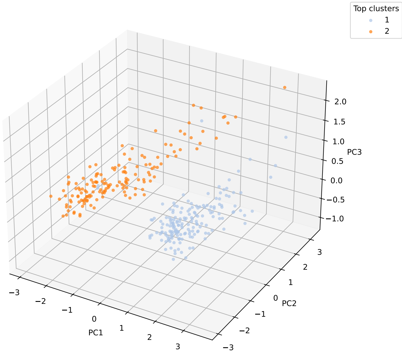
Clusters in 3-D PCA space (EVR: 0.56, 0.35, 0.05)
