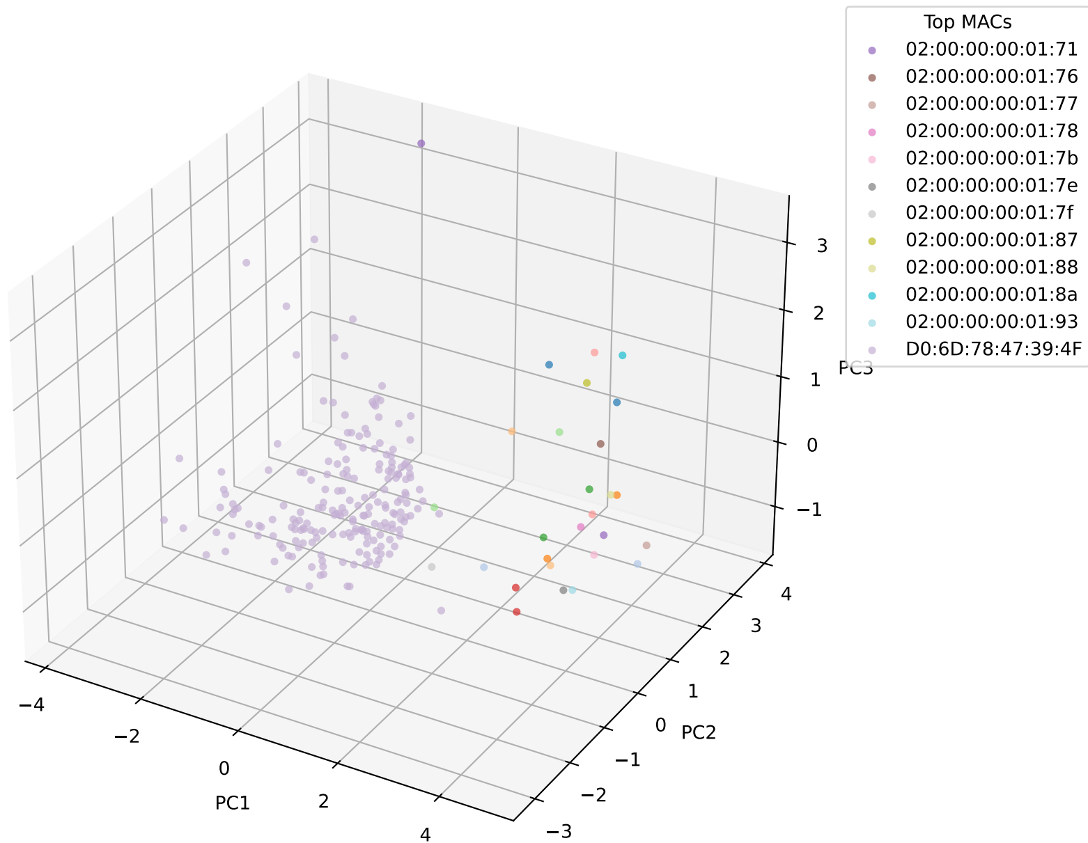
MAC-colored 3-D PCA of CFO (EVR: 0.48, 0.37, 0.09)
