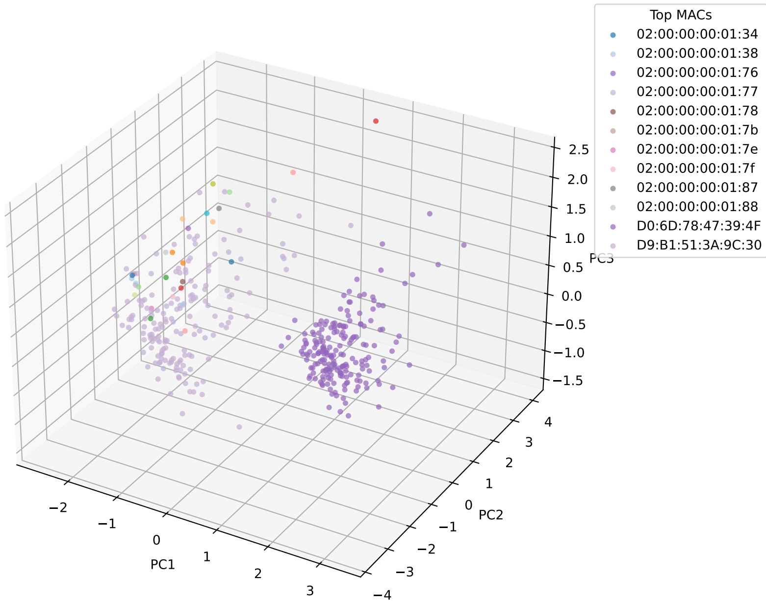
MAC-colored 3-D PCA of CFO (EVR: 0.53, 0.38, 0.06)
