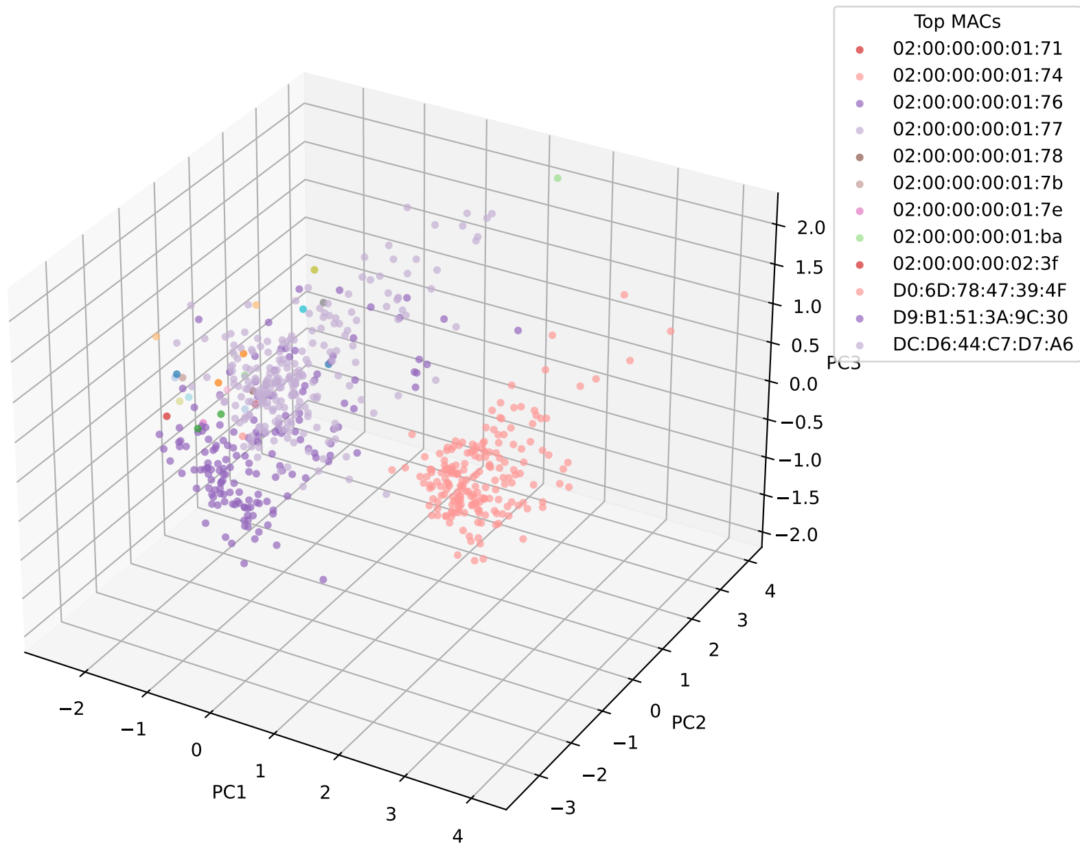
MAC-colored 3-D PCA of CFO (EVR: 0.50, 0.35, 0.09)
