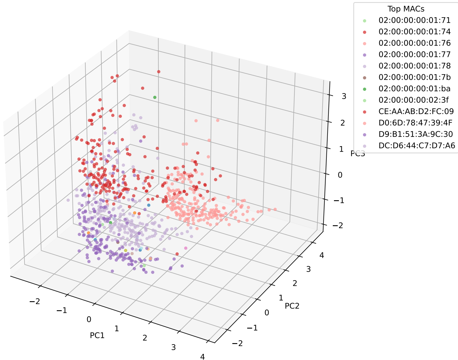
MAC-colored 3-D PCA of CFO (EVR: 0.38, 0.34, 0.22)
