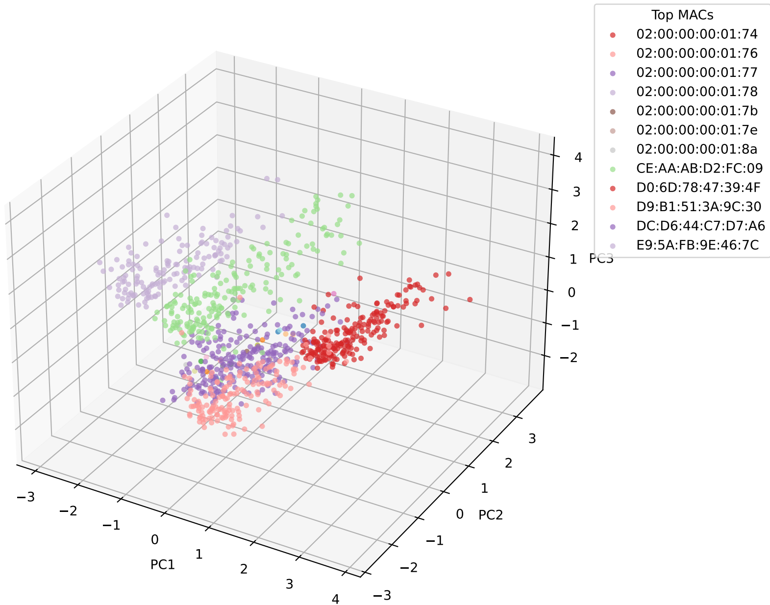
MAC-colored 3-D PCA of CFO (EVR: 0.37, 0.31, 0.25)
