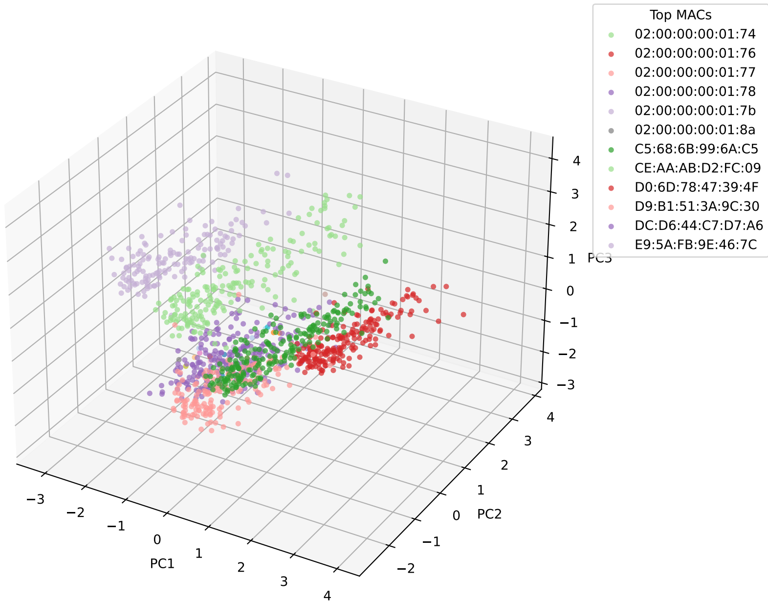
MAC-colored 3-D PCA of CFO (EVR: 0.36, 0.32, 0.24)
