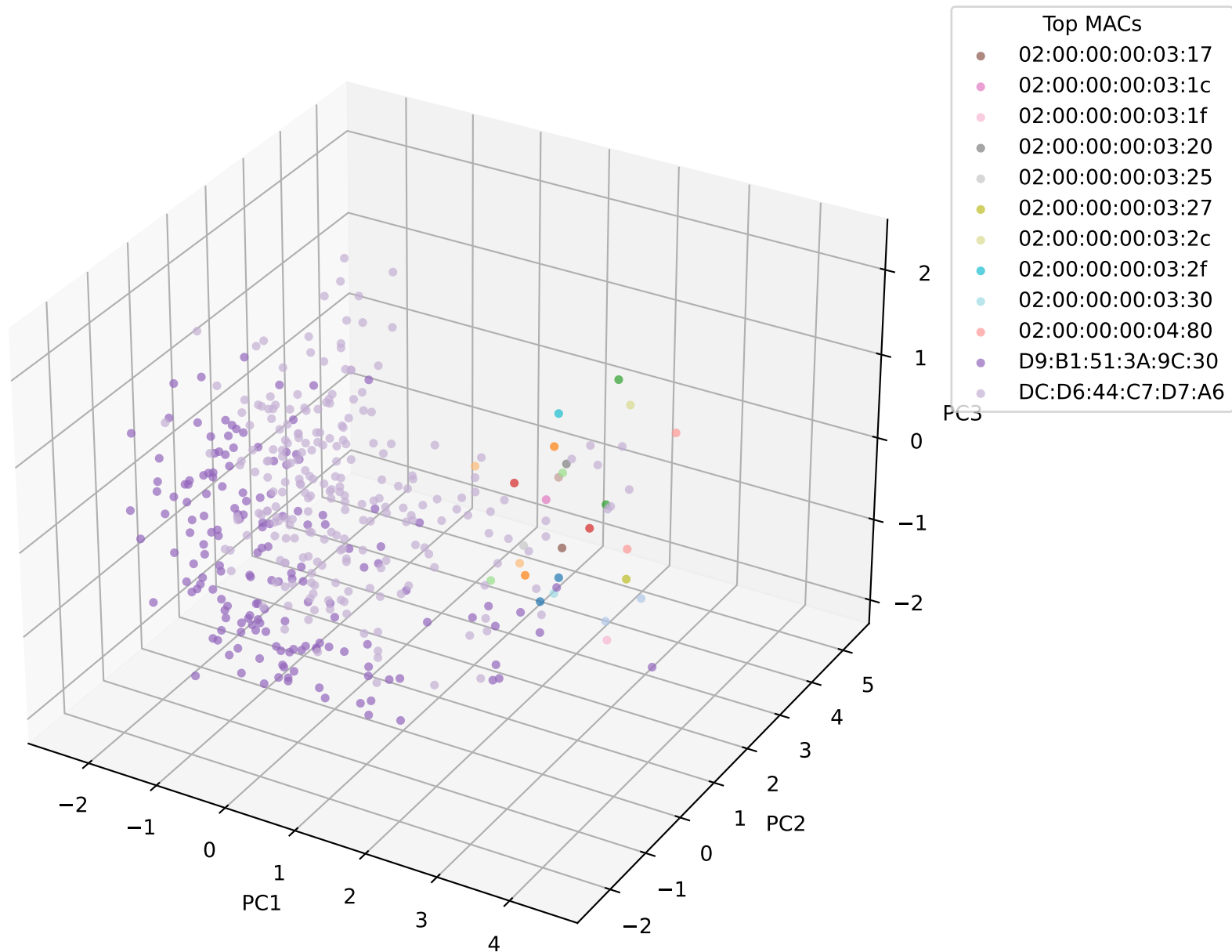
MAC-colored 3-D PCA of CFO (EVR: 0.39, 0.35, 0.16)
