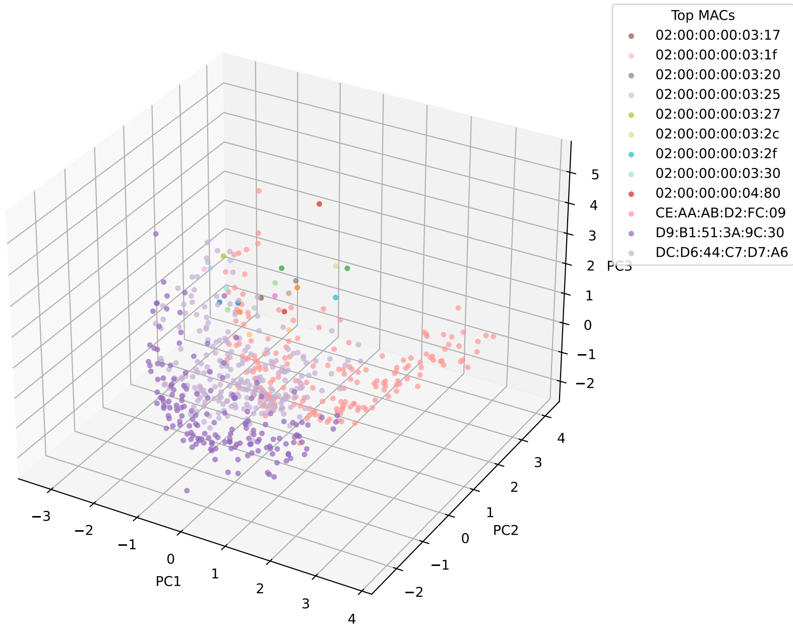
MAC-colored 3-D PCA of CFO (EVR: 0.38, 0.33, 0.22)
